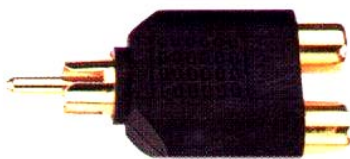
JX3073 RCA MALE TO 2 X RCA FEMALE A = GOLD , B = NICKEL
