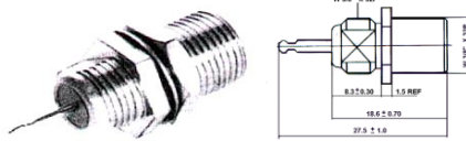
JX2097 "F" FEMALE BULKHEAD WITH NUTS
